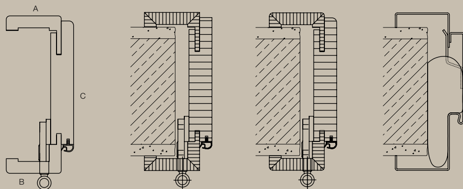
A: Decorative edge Timber frame, angular Timber frame, round edge Steel profile frame VarioFix B: Rebate cladding C: Jamb lining
