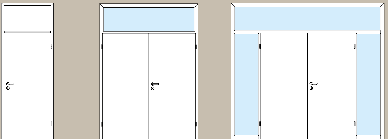
Single-leaf, 1 transom panel, alternatively also with transom light
