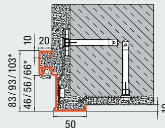
Corner frame with plug-and-screw fitting (Brickwork/concrete)
