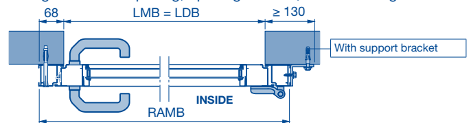
Fitting behind the opening, opening inwards, RH or LH hinged
