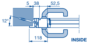
Profile type 2 (opening inwards)
