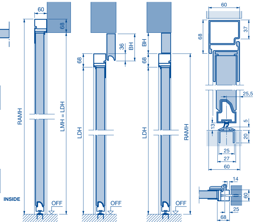
Profile type 1/2 Panel in front of the side door
